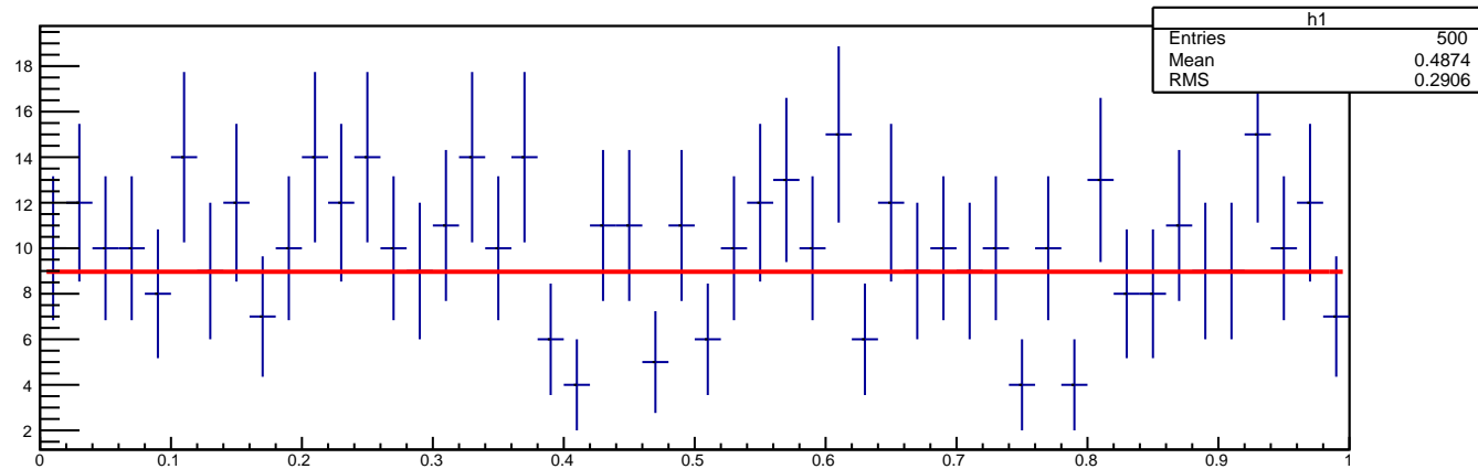
AD Test using R package kSamples
