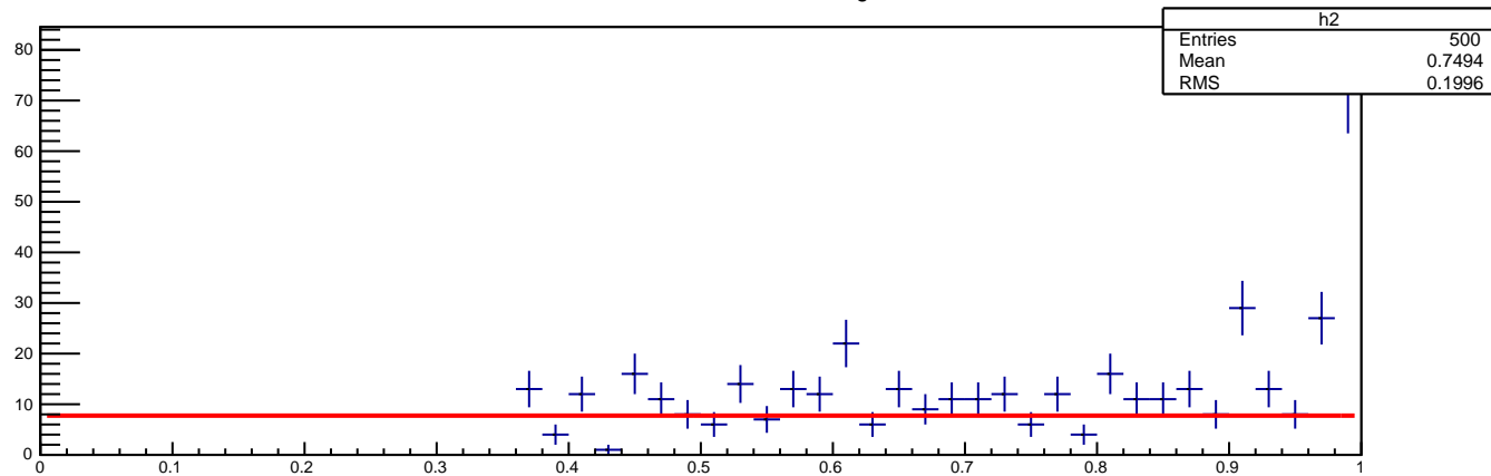
AD Test using ROOT::Math::GoFTest
